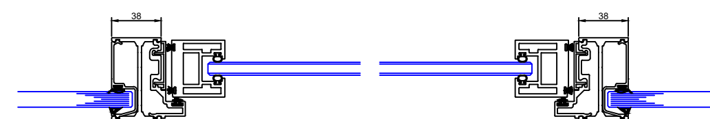
Single Glazed Micro Framed Door to Single Glazing
