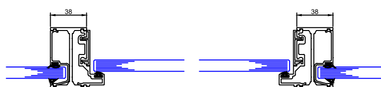
Single Glazed Door to Single Glazing
