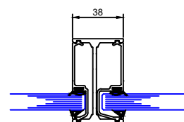
Single Glazed Mullion
