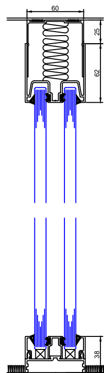
Double Glazing with Deflection Head & Base Sections
