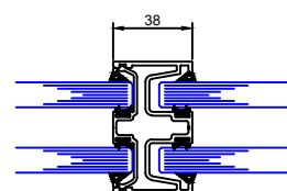
Double Glazed Mullion
