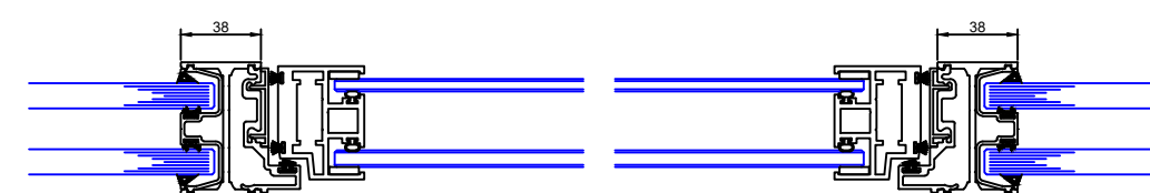
Double Glazed 54mm Rebated Framed Door to Double Glazing
