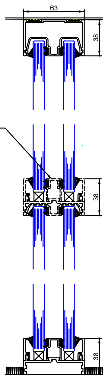
Double Glazing with Standard Head & Base Sections
