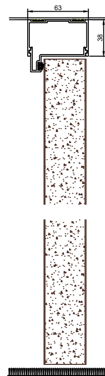
Timber Door Standard Head Section
