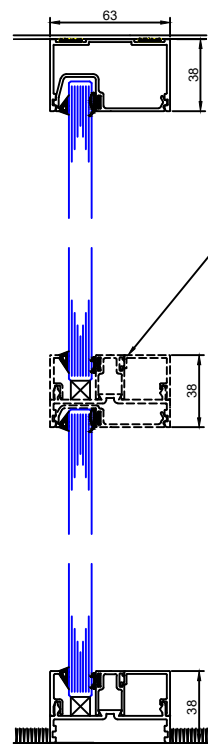
Single Glazing with Standard Head & Base Sections
