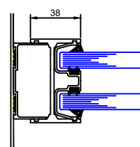
Double Glazed Deflection Abutment
