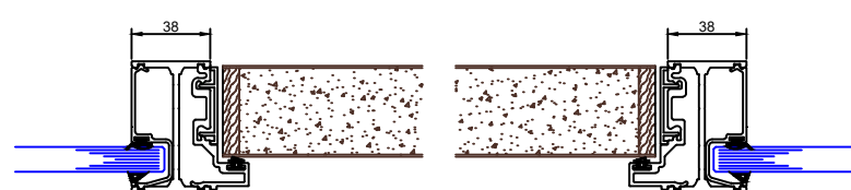
Timber Door to Single Glazing
