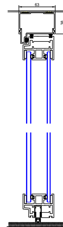
54mm Rebated Double Glazed Door with Standard Head Section
