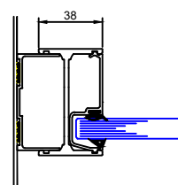
Single Glazed Deflection Abutment
