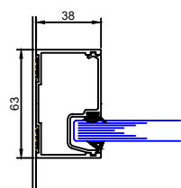
Single Glazed Abutment
