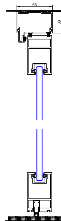
Wide Framed Single Glazed Door with Standard Head Section
