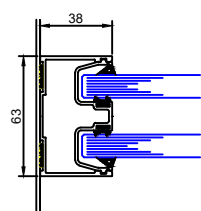
Double Glazed Abutment
