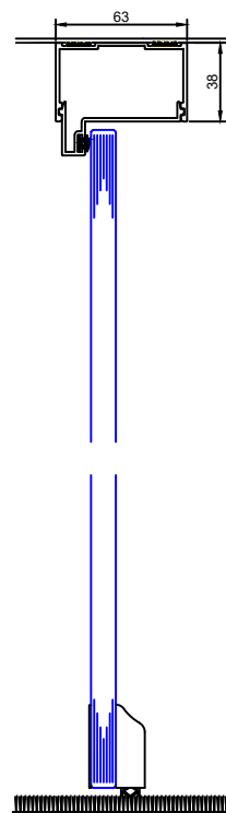
Single Glazed Door Standard Head Section
