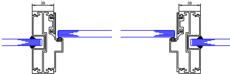
Single Glazed Door to Single Glazing
