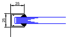
25mm Abutment
