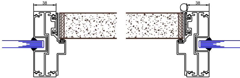
Timber Door to Single Glazing
