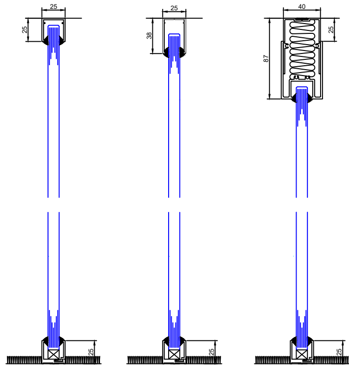
Single Glazing with Minimal Head & Base Sections Single Glazing with 38mm Head & 25mm Base Sections Single Glazing with Deflection Head & 25mm Base Sections
