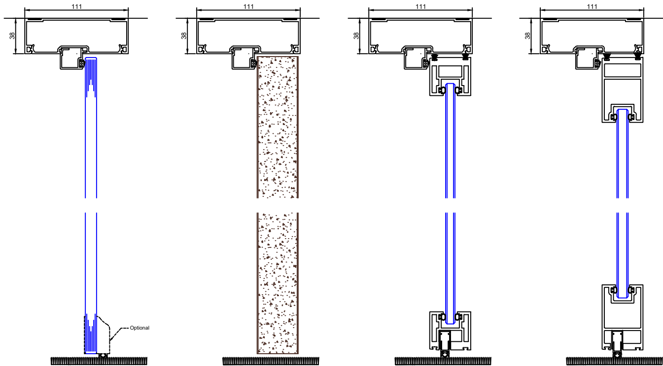
Single Glazed Door Standard Head Section Timber Door Standard Head Section Single Glazed Door with Standard Head Section Wide Framed Door with Standard Head Section
