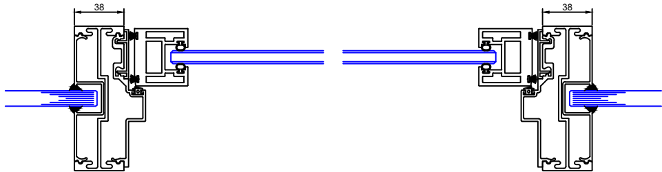
Single Glazed Micro framed Door to Single Glazing
