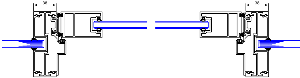
Wide Framed Glazed Door to Single Glazing
