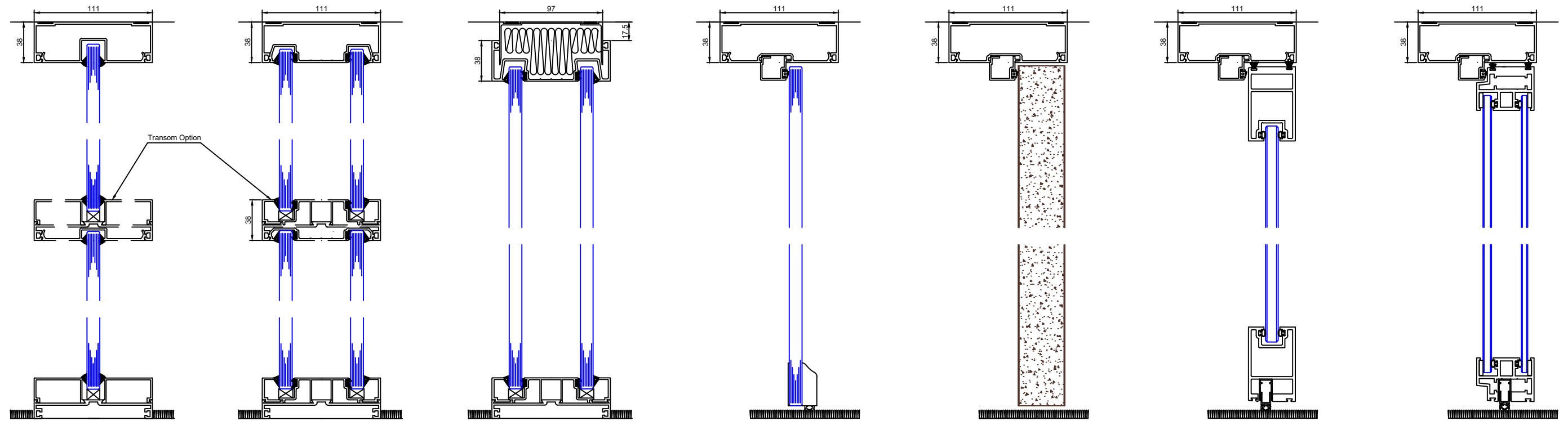
Single Glazing with Standard Head & Base Sections
