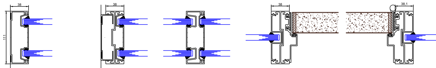
Double Glazed Abutment
