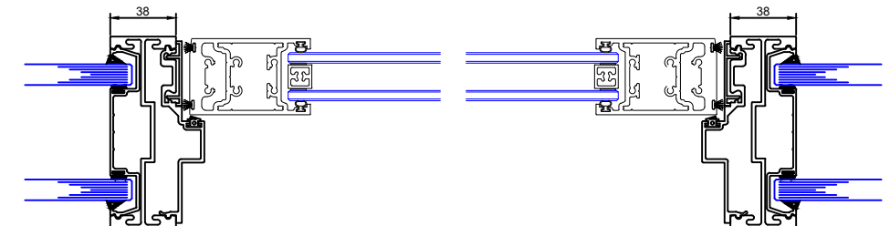
Double Glazed Wide Framed Door to Double Glazing
